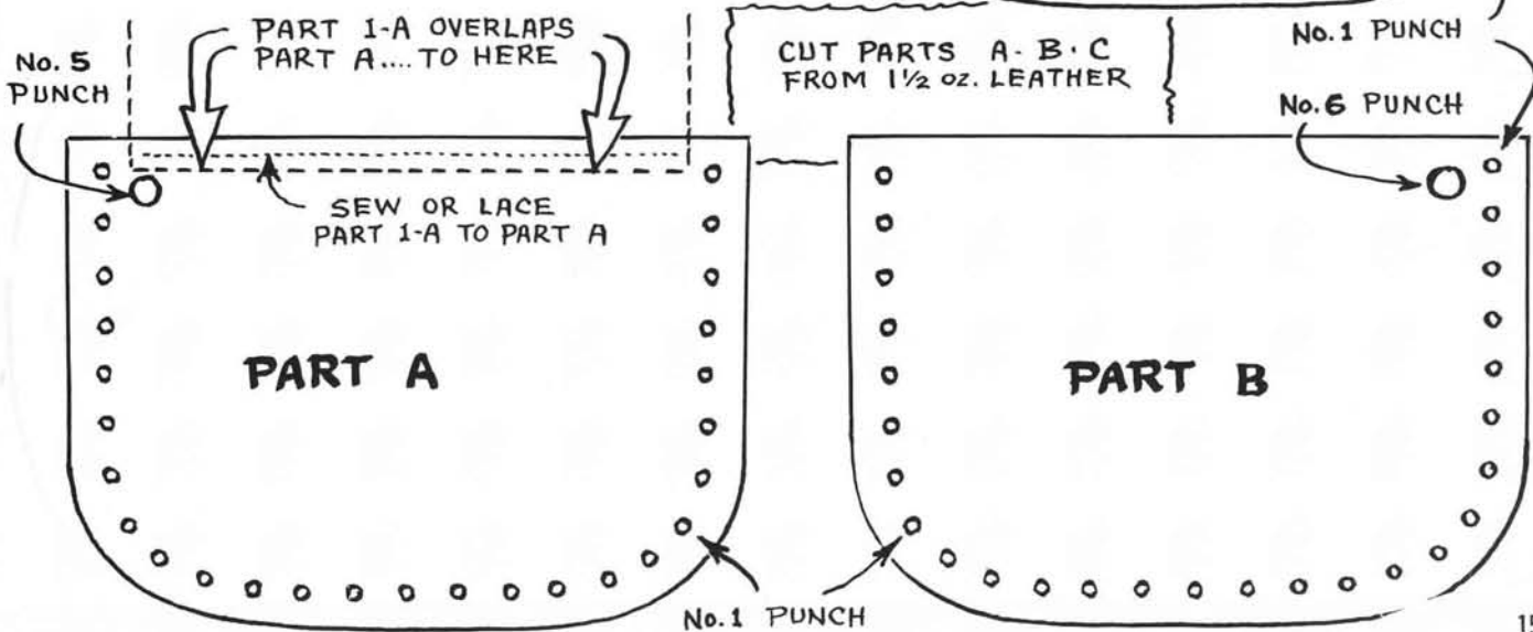
PART 1-A CUT FROM 3 oz. CALF OR COWHIDE
