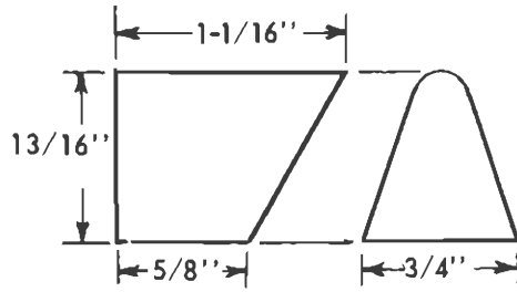
WOODEN SUPPORT
